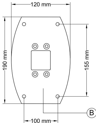
Holes Pattern SMS Projector WL V Wall Plate
