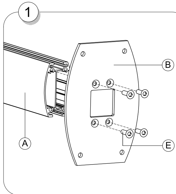
Holes Pattern SMS Projector WL V Wall Plate
